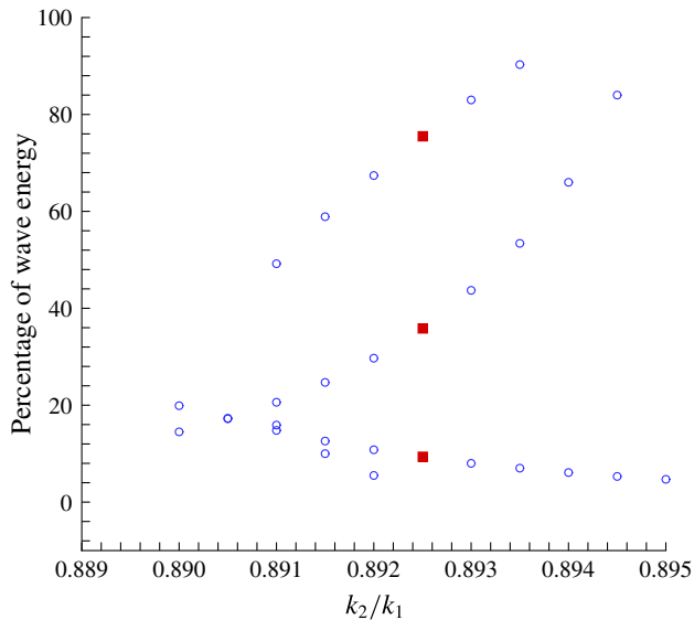
FIGURE 6. (Colour online) Wave energy distribution (%) obtained by Zakharov equation of the wave component \mathbf{k}_3 = 2\mathbf{k}_1 - \mathbf{k}_2 of the steady-state exactly and nearly resonant wave system in the case of \sigma_1/\sqrt{gk_1} = \sigma_2/\sqrt{gk_2} = \epsilon = 1.0003 with various k_2/k_1 , when the angle between wavenumbers \mathbf{k}_1 and \mathbf{k}_2 of the two primary waves is \pi/36 . The filled squares correspond to the exactly resonant wave.
