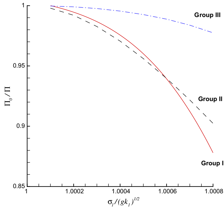
Fig. 10. \Pi_0/\Pi versus \sigma_1/\sqrt{gk_1} in case of (65) when k_2/k_1 = 0.8925 and \sigma_1/\sqrt{gk_1} = \sigma_2/\sqrt{gk_2} for different group of solutions. Solid line: Group I. Dashed line: Group II. Dash-dotted line: Group III.
