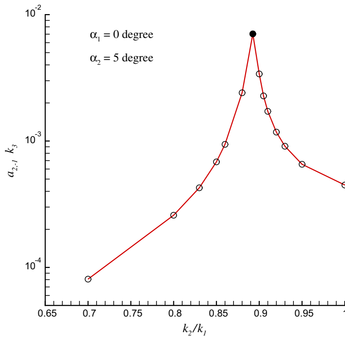
Fig. 6. The dimensionless wave amplitude component k_3(a_{2,-1}) versus k_2/k_1 in case of (65). Filled circle: result when k_2/k_1 = 0.8925 . Open circles: results when k_2/k_1 \neq 0.8925 .
