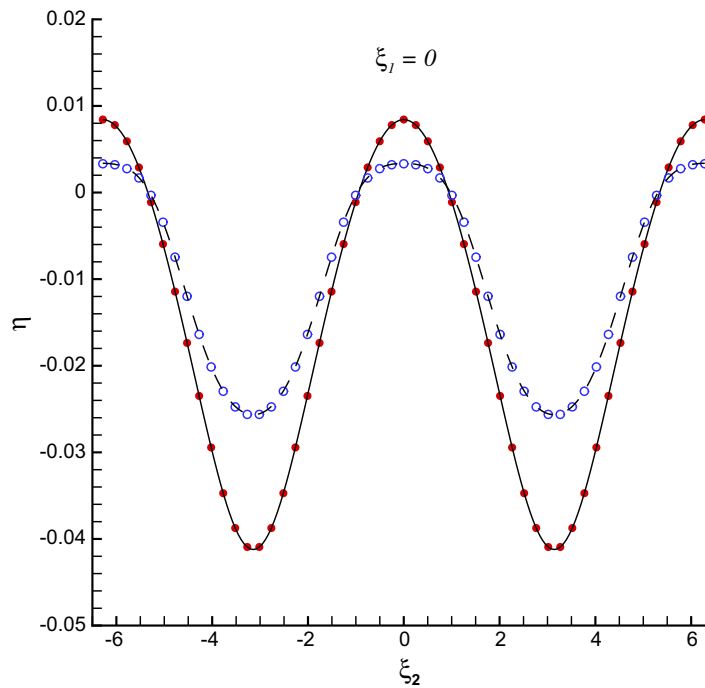
Fig. 8. Resonant wave profile at \xi_1 = 0 in case of (65) with k_2/k_1 = 0.8925 . Solid line: the 10th-order of approximation of Group II. Dashed line: the 10th-order of approximation of Group III. Symbols: 6th-order approximations.
