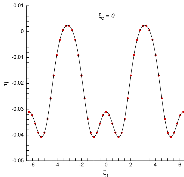
Fig. 4. Resonant wave profile at \xi_2 = 0 in case of (65) with k_2/k_1 = 0.8925 . Symbols: 5th-order approximation. Solid line: 10th-order approximation.
