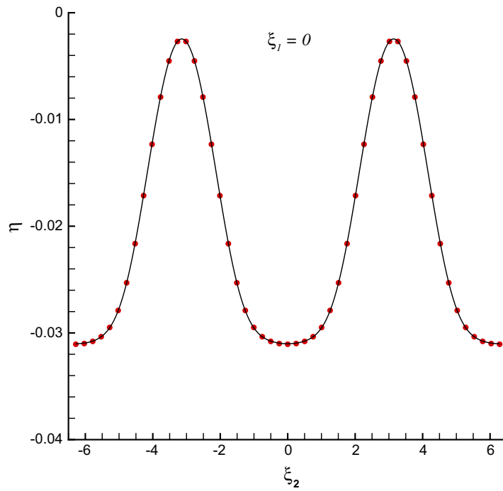
Fig. 5. Resonant wave profile at \xi_1 = 0 in case of (65) with k_2/k_1 = 0.8925 . Symbols: 5th-order approximation. Solid line: 10th-order approximation.
