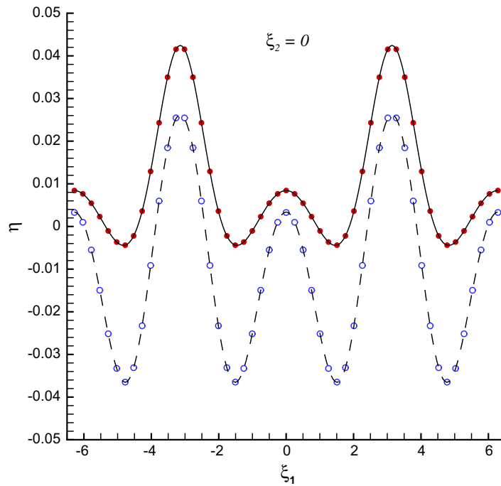
Fig. 7. Resonant wave profile at \xi_2 = 0 in case of (65) with k_2/k_1 = 0.8925 . Solid line: the 10th-order of approximation of Group II. Dashed line: the 10th-order of approximation of Group III. Symbols: 6th-order approximations.
