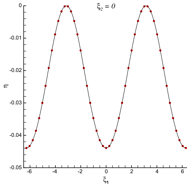
Fig. 2. Wave profile at \xi_2 = 0 in case of (65) with k_2/k_1 = 1 . Symbols: 3rd-order approximation. Solid line: 10th-order approximation.
