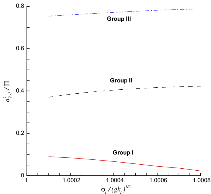
Fig. 9. a_{2,-1}^2/\Pi versus \sigma_1/\sqrt{gk_1} in case of (65) when k_2/k_1 = 0.8925 and \sigma_1/\sqrt{gk_1} = \sigma_2/\sqrt{gk_2} for different group of solutions. Solid line: Group I. Dashed line: Group II. Dash-dotted line: Group III.
