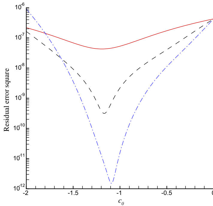
Fig. 3. Residual error square versus the convergence-control parameter c_0 in case of (65) with k_2/k_1 = 0.8925 . Solid line: 1st-order approximation. Dashed line: 3rd-order approximation. Dash-dotted line: 5th-order approximation.
